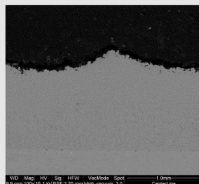
SST-A5001 Coating on Al6061 (Series EP)
